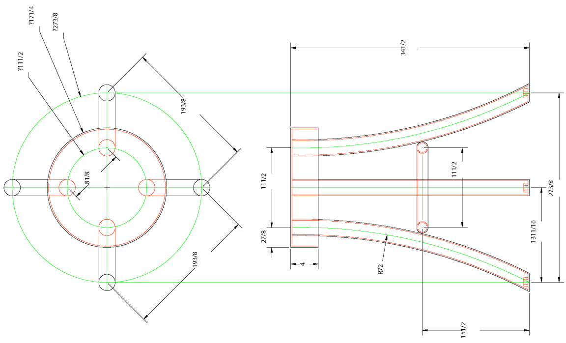
SECTION A-A BACKREST NOT SHOWN FOR CLARITY
